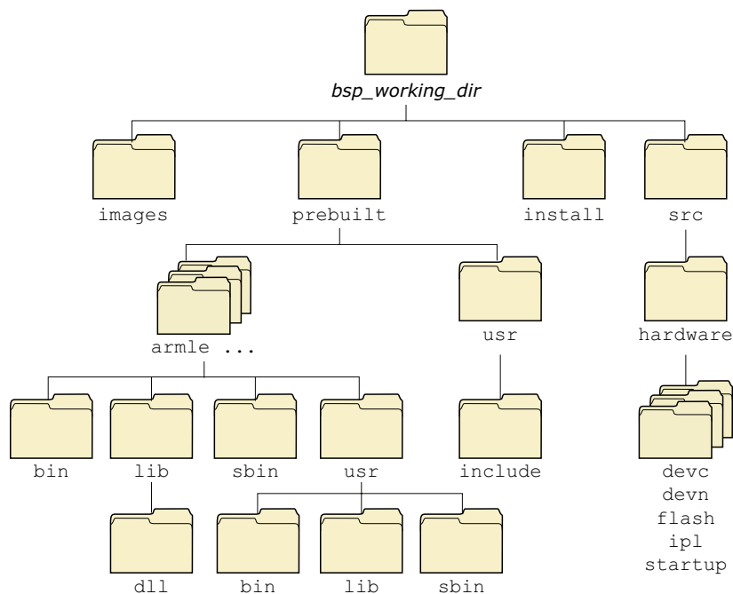
BSP directory tree.
